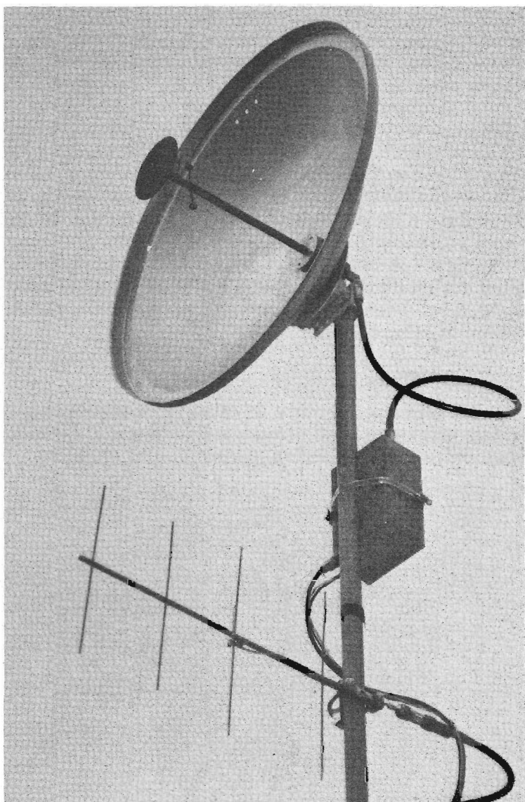
Fig. 4-5. A portable repeater system using 434-MHz input and 1277-MHz ATV transmitter. This system was used for coverage of the Pasadena Rose Parade.
