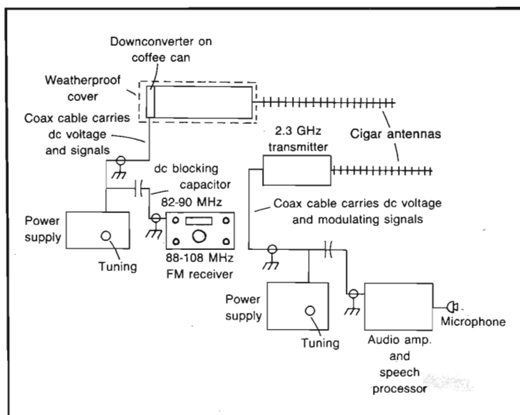
Fig. 5-1. An amateur transceiving setup for voice communications on 2.3 GHz. Although a conventional FM receiver is shown for reception, a more narrow-band i-f system may be used.
