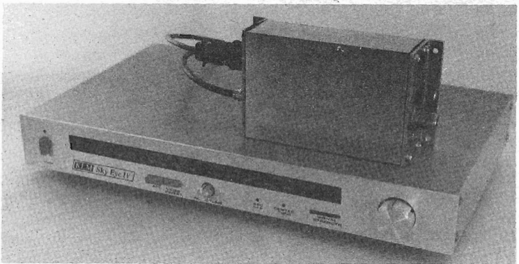
Fig. 12-5. The KLM Sky Eye IV satellite TV receiver, with remote downconverter on top of the unit. This is a state-of-the-art unit priced in the range of many familiar Amateur Radio high-frequency transceivers (courtesy KLM Electronics, Morgan Hill, California).
