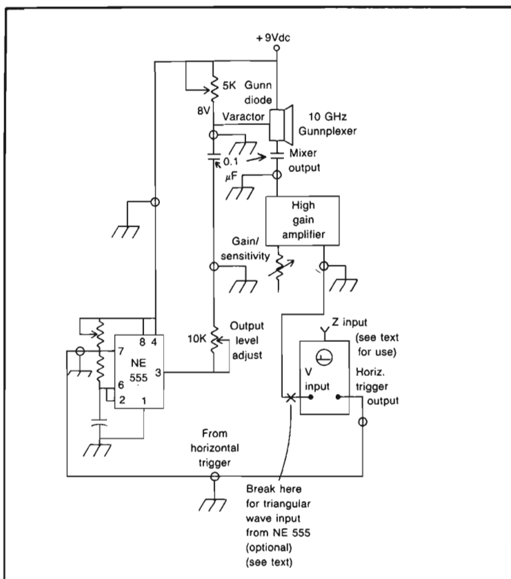
Fig. 11-5. Block diagram of the first generation amateur weather RADAR system by K4TWJ. The Gunnplexer transmits and receives 10-GHz energy, and the oscilloscope provides timing and range information.
