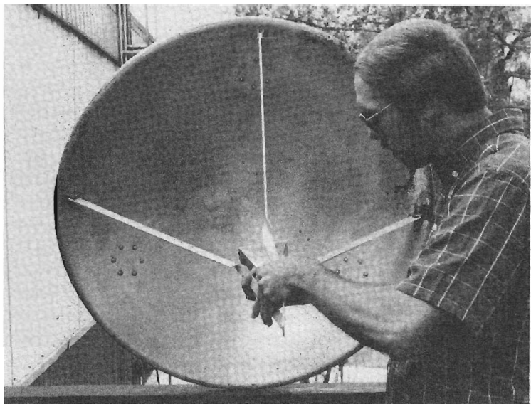
Fig. 1-5. Author Dave Ingram, K4TWJ, makes preliminary focal-point adjustments in a 10-GHz Gunnplexer and 3.5-foot dish antenna to be used in a microwave link. The system is capable of relaying amateur high-frequency band signals or amateur television (ATV) signals.
