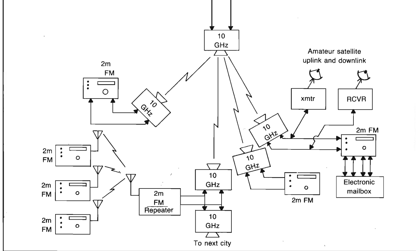
Fig. 1-1. Simplified overview of a basic microwave network that can be expanded to cover many areas and modes.
