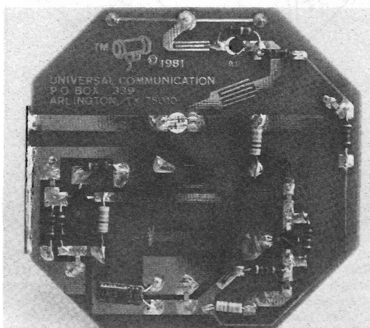
Fig. 3-6. A full view of the 2-GHz downconverter shown in Fig. 3-5. The rf amplifier is at the top, mixer diodes near the middle, local oscillator at the left bottom, and the i-f amplifier is at the right bottom.
