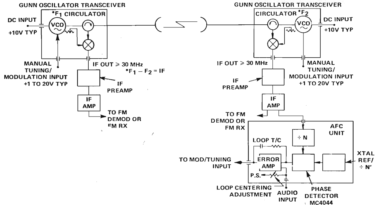
Fig. 3-9. A method of applying digital automatic frequency control (courtesy Microwave Associates).
