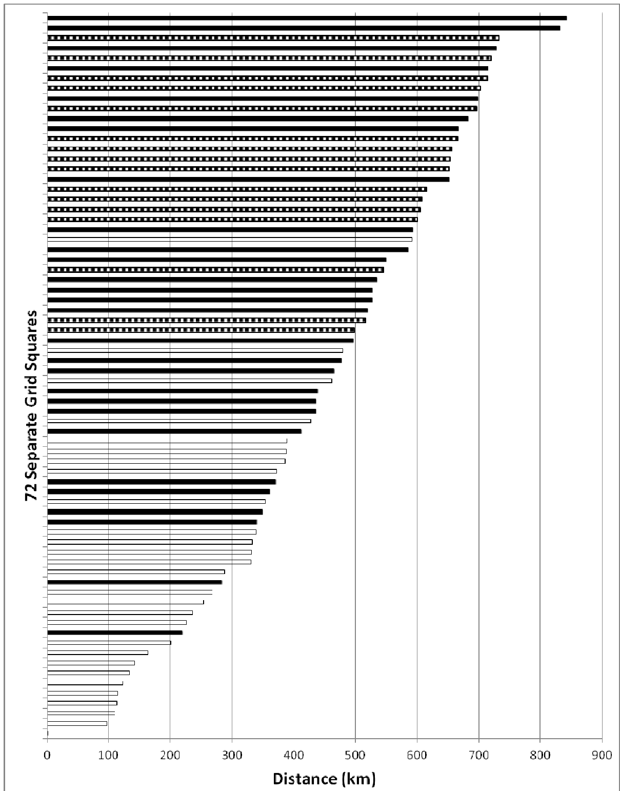
Figure 2 – Operating Mode versus Distance for 10 GHz. Black is JT65c broken is ISCAT-A and unfilled is SSB Where a contact was first completed on a Digital Mode and latter on SSB the chart indicates SSB to show SSB was possible.
